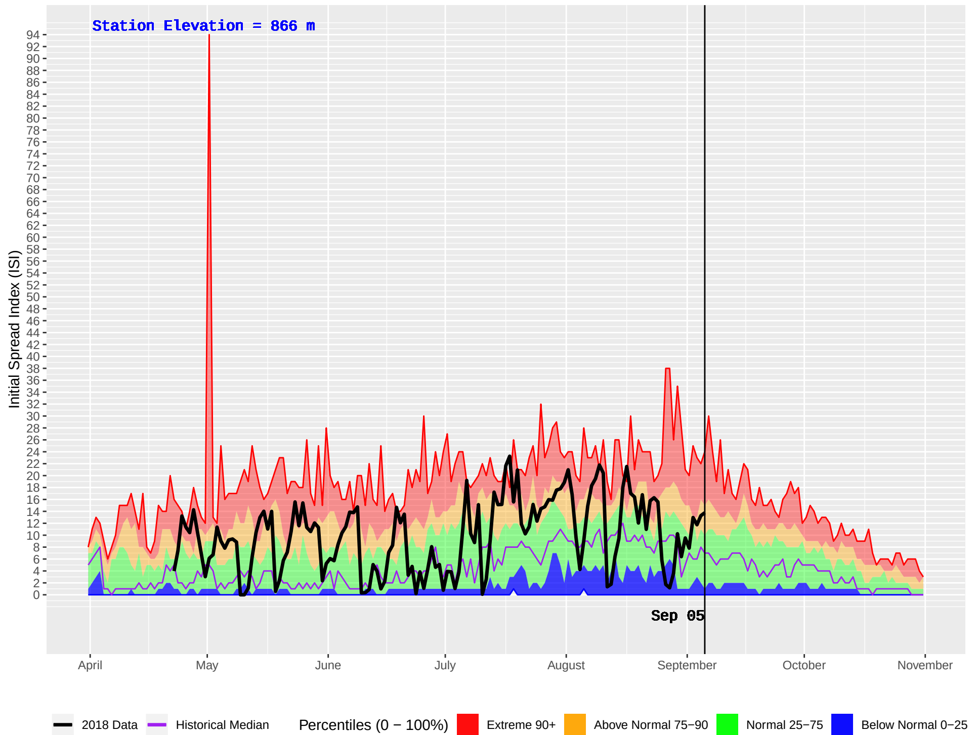
NICOLL (393) : Historical (1981–2016) and Current (2018) Daily Initial Spread Index (ISI)
