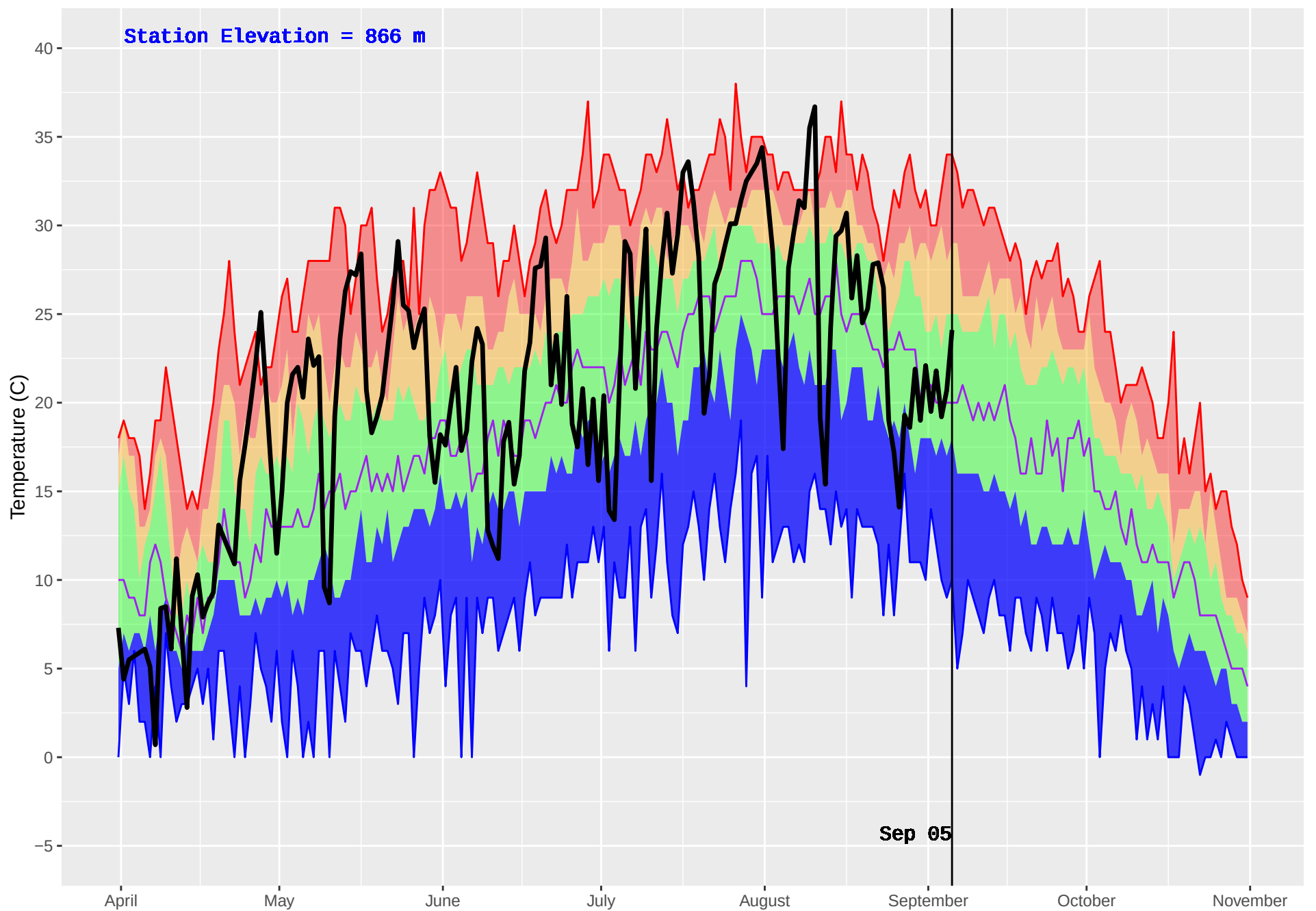
NICOLL (393) : Historical (1981–2016) and Current (2018) Daily Temperature
